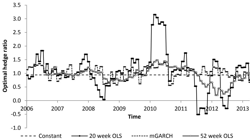
Figure 1: Constant and optimal hedge ratios
